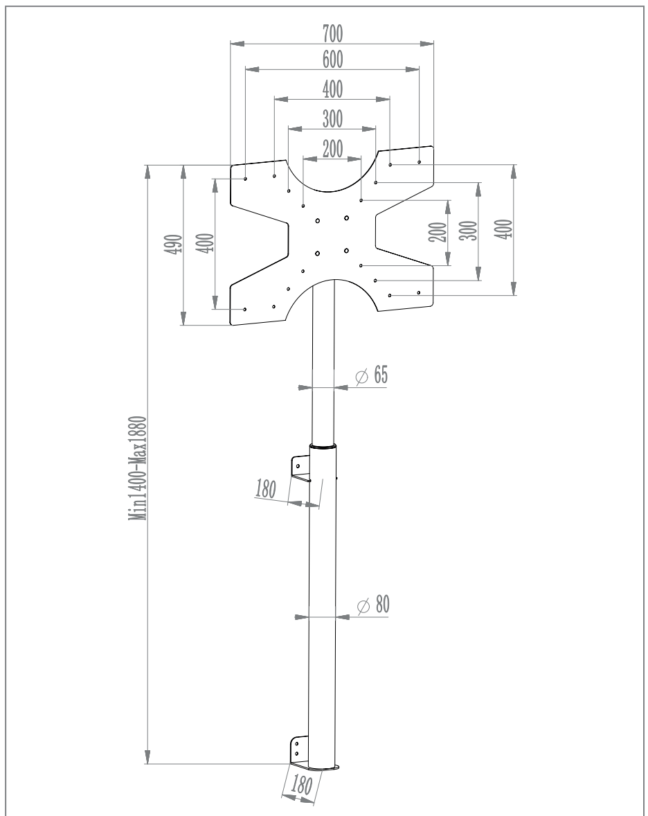
Optional: Braclabs Stand Front shelf (Item no.: 1984)
